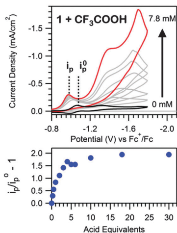
Fig. 1 Top: voltammograms of 0.39 mM 1 with additions of 0 to 20 eq. (7.8 mM) of CF 3 COOH at 100 mV s -1 in a 100 mM [Bu 4 N][PF 6 ] CH 3 CN solution. Bottom: the peak current of the prewave relative to the one-electron reduction of the catalyst in the absence of acid ( i_p = peak current, i_p^0 = peak current of Ni^{II}/Ni^I reduction in absence of acid).
