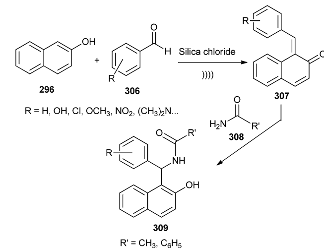
Scheme 65 Synthesis of amidoalkyl naphthols.
