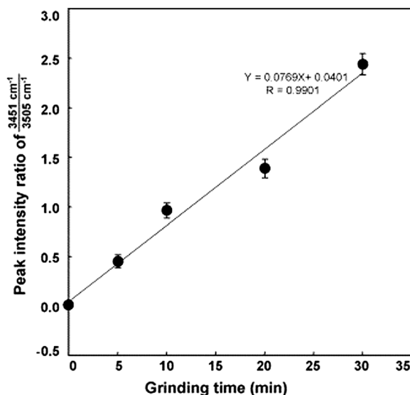
Fig. 6 (a) Grinding-time dependence of the FTIR spectra for famotidine showing from top to bottom the emergence of the absorption at 3451 cm⁻¹ which is used to monitor the formation of Form A of the material. (b) Plot of peak intensity ratio ( I_{3451}/I_{3505} ) for the spectra above indicating a possible zero order rate law for the conversion. Reproduced from ref. 78 with permission from Elsevier.
