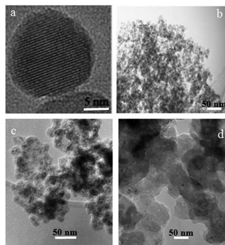
Fig. 3 TEM images of (a) \gamma\text{-Fe}_2\text{O}_3 MNPs 1 , (c) iodoalkyl-functionalized \text{SiO}_2 -coated MNPs 3 and (d) neocuproine functionalized MNPs 7 .
