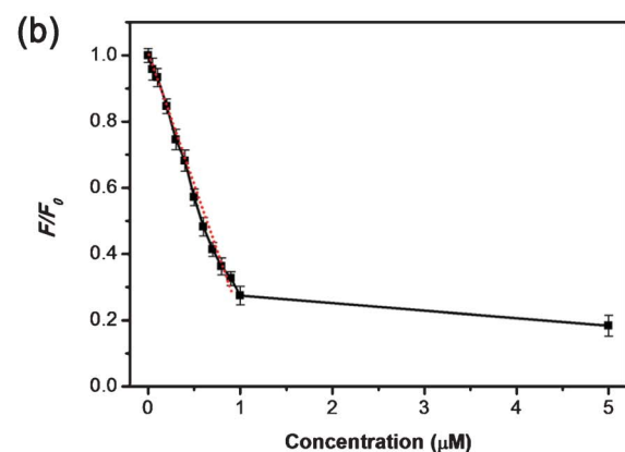
Fig. 5 (a) PL spectra of GCQD aqueous solutions with different \text{Fe}^{3+} concentrations (from top to bottom: 0, 2, 50, 100, 200, 300, 400, 500, 600, 700, 800, 900 nM, 1 and 5 \mu\text{M} , respectively). (b) The dependence of F/F_0 on the concentration of \text{Fe}^{3+} ions within the range of 0–5 \mu\text{M} . The excitation wavelength was fixed at 340 nm for all the PL spectra. F and F_0 are the PL intensities at 445 nm in the presence and absence of \text{Fe}^{3+} ions, respectively.
