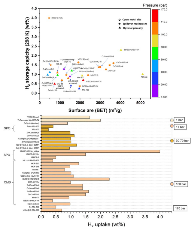
Fig. 11 Comparison of the H_2 storage capacities of different types of MOFs concerning surface area and pressure at RT.
