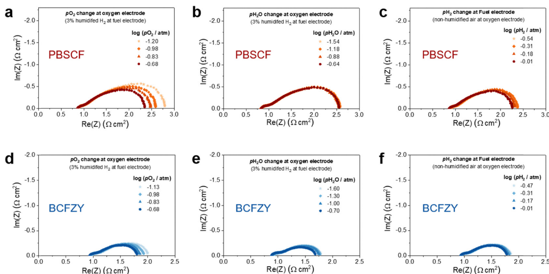
Fig. 5 Electrochemical impedance spectra (Nyquist plots) of PCFCs with PBSCF (top row) and BCFZY (bottom row) cathodes measured at 550 \text{ }^\circ\text{C} under different gas conditions. (a and d) Effect of varying pO_2 at the cathode, (b and e) effect of pH_2O at the cathode (with a constant flow of 3% humidified H_2 at the anode), and (c and f) effect of pH_2 at the anode (with a constant flow of dry air at the cathode). Nyquist plots correspond to PBSCF (a–c) and BCFZY (d–f) cathodes, respectively.
