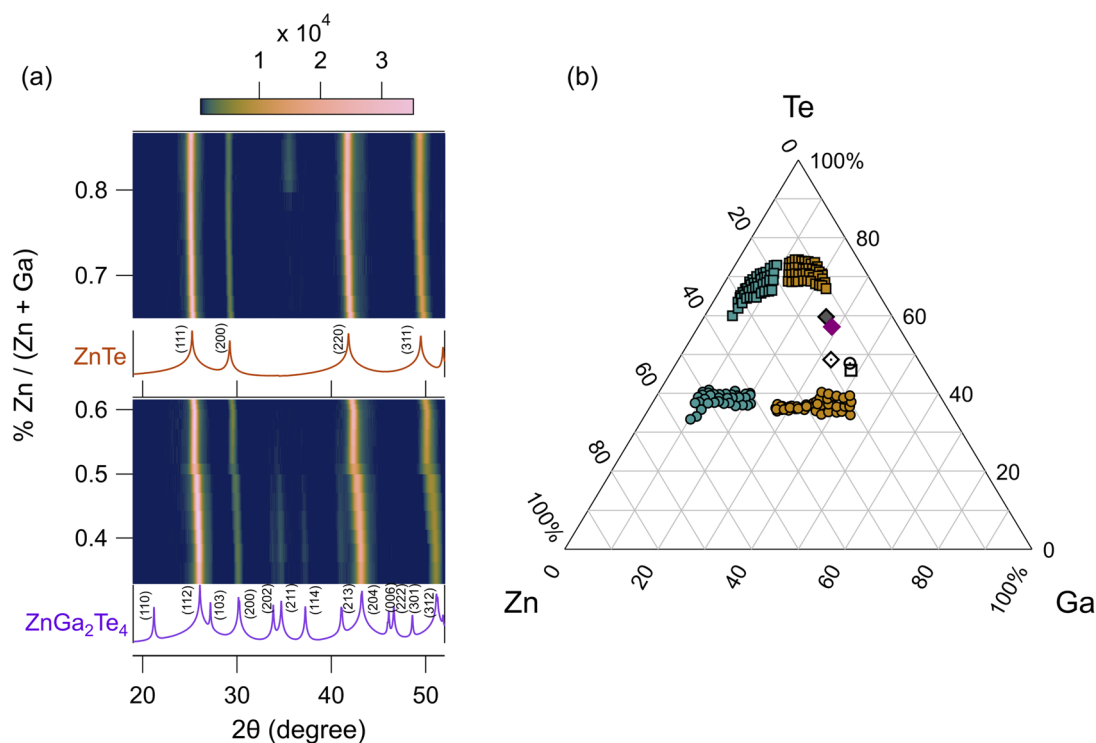
Fig. 2 Structural characterization (a) diffraction heatmap from post annealed samples ( T_{\text{growth}} \sim 500 °C) that exhibit the cubic (upper panel)–tetragonal (lower panel) crystal symmetry ( \lambda = 1.54 Å) (b) ternary phase diagram showing the full composition of films (filled square and circle shape represents as-deposited sample and annealed samples, respectively) on EXG glass. Filled diamond shape (magenta) represent nominal stoichiometric \text{ZnGa}_2\text{Te}_4 composition. Other symbols represent the \text{ZnGa}_2\text{Te}_4 composition synthesized on FTO glass for photoelectrochemical measurement.
