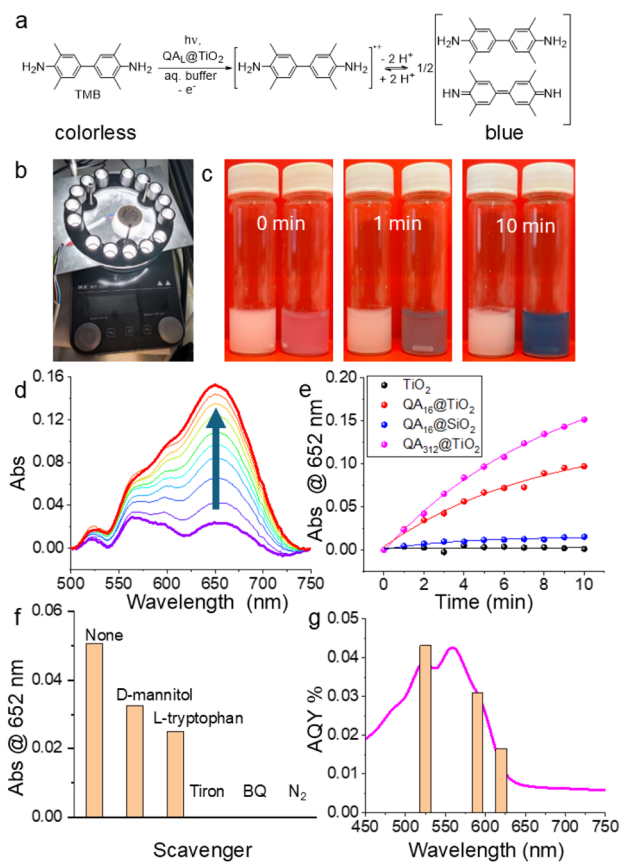
Fig. 2 (a) Light driven oxidation of 0.2 mM TMB with 1 mg per mL QA L @TiO 2 NPs in 2 mL of 0.1 M aqueous acetate buffer, pH 5. (b and c) Images of the photoreactor and of the reaction vials over ten minutes containing QA 312 @TiO 2 (right) and TiO 2 control (left). (d) Spectral evolution obtained for photochemical oxidation of TMB with QA 312 @TiO 2 NPs. (e) Plot of the absorbance at 652 nm over time for the NPs investigated. The spectroscopic response was recorded with a plate reader, sampling aliquots of 100 \mu L of the irradiated solution every minute. (f) Control tests in the presence of scavengers (7.5 mM); the absorbance at 652 nm reported in the histograms refers to the QA 16 @TiO 2 particles after 4 minutes irradiation. (g) Apparent Quantum Yield (AQY%) superimposed to the diffuse reflectance spectrum of QA 312 @TiO 2 NPs.
