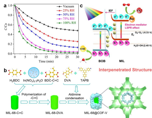
Fig. 13 (a) Photocatalytic \text{CH}_3\text{CHO} degradation rate curves over \text{UCNP/NMIL}(\text{Ti}) under visible light with different RH%. 92 Copyright 2022, Elsevier. (b) The construction process of \text{MIL-68@COF-V} . 135 Copyright 2024, John Wiley and Sons. (c) Photocatalytic mechanism of the plasmonic S-scheme heterojunction in \text{Au/MIL/BOB} . 160 Copyright 2024, Elsevier.
