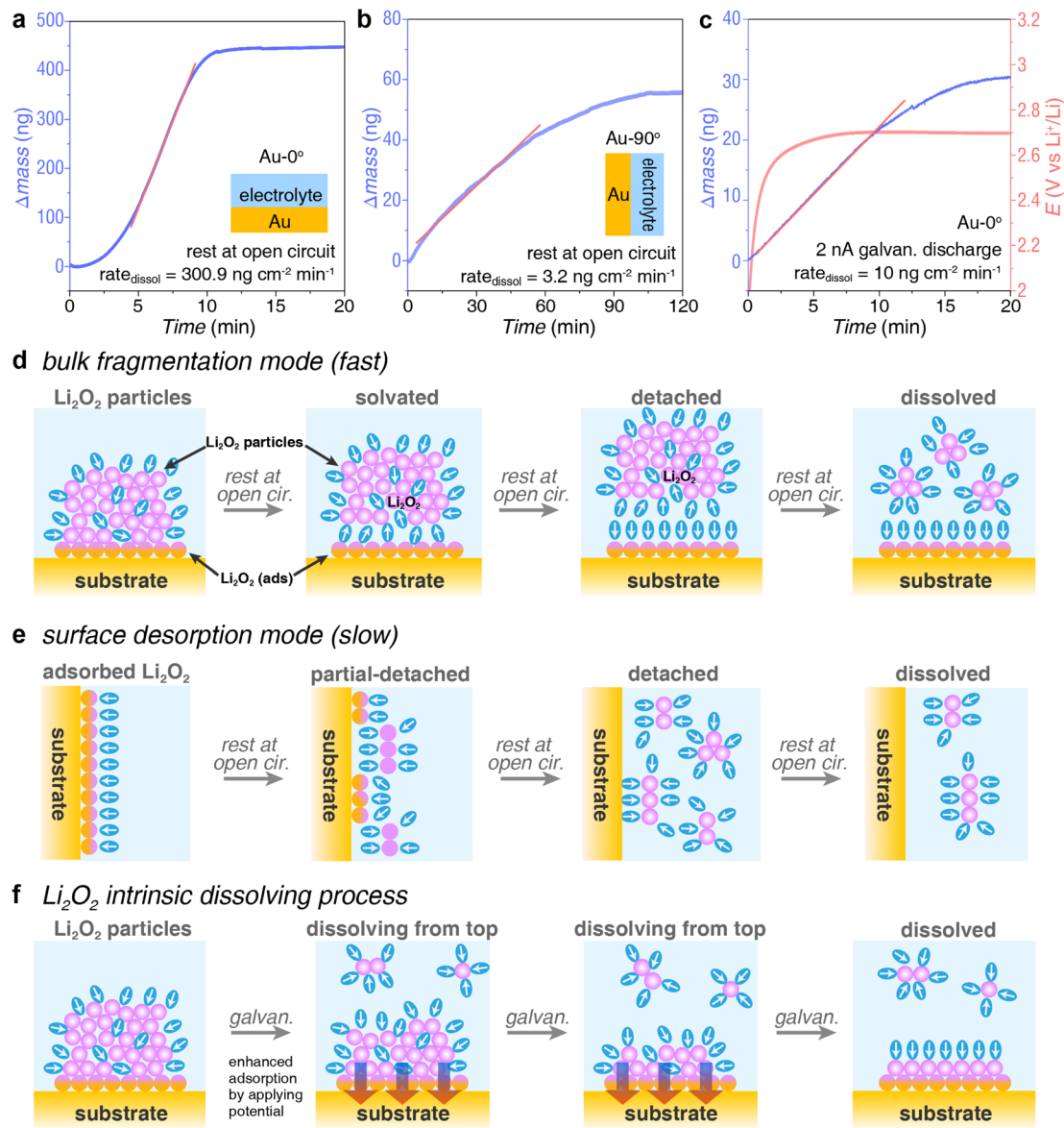
Fig. 4 Kinetics of dissolution process of Li_2O_2 . (a and b) Rate of natural dissolution of Li_2O_2 that was deposited on (a) Au-0° electrode and (b) Au-90° electrode at open circuit. (c) Rate of Li_2O_2 dissolution on Au-0° electrode at a reduction potential to maintain surface adsorption. A tiny discharging current of 2 nA (equivalent to 0.12 \text{ ng}_{Li_2O_2} \text{ cm}^{-2} \text{ min}^{-1} deposition) was applied to keep the cell under a discharging status. (d–f) Schematics of the various dissolving processes corresponding to EQCM results in a–c.
