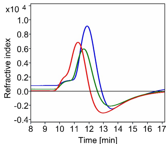
Fig. 4 SEC analysis of the functionalized α-PLLs 12b (●), 12db (●), and 12e (●). Eluent: 150 mM phosphate buffer with 750 mM NaCl at pH = 6.8; flow rate: 0.5 mL min -1 ; temperature: 35 °C.
