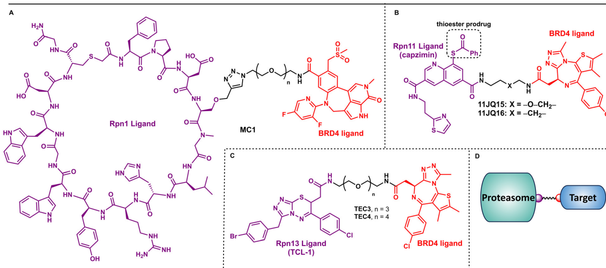
Fig. 7 A. Peptidic macrocycle (MC1) is a ligand for Rpn1 that, when connected to a BRD4 (BET1) ligand through a PEG linker installed via click chemistry, can degrade BRD4. B. Two RPN11 ligand-based bifunctional molecules can successfully degrade BRD4 in a proteasome dependent manner. C. Non-covalent ligand for Rpn13 (TCL-1) was also elaborated into a BRD4 bifunctional degrader. D. A, B, and C all aim to affect degradation via direct recruitment to the proteasome and bypass the need for E3 recruitment and ubiquitination.
