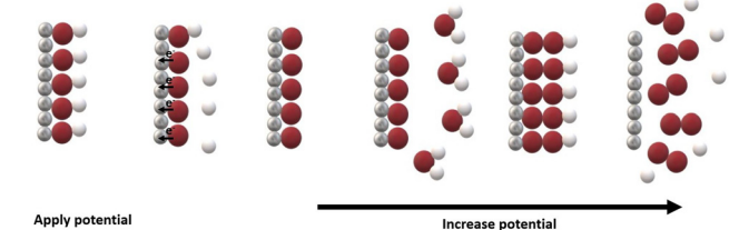
Fig. 7 OER mechanism as described by Rossmeisl and Nørskov. 46 Silver: metal surface; red: oxygen; white: hydrogen. When a potential is applied, water molecules dissociate and form OH ad (eqn (13)). Without a further increase in potential, a proton is split off into solution and an electron to the electrode (eqn (14)). After this, the coverage of O ad increases until no new OH ad forms. If the potential is high enough, water molecules will adsorb on O ad , forming OOH ad (eqn (15)) and eventually evolve O 2 (eqn (16)).
