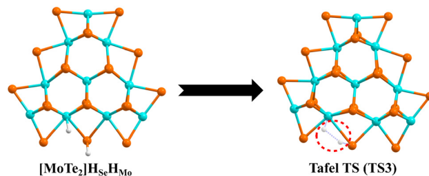
Fig. 7 The Volmer–Tafel reaction mechanism equilibrium geometries of [MoTe_2]H_xH_x^{-1} and TS3 are shown here.
