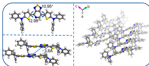
Fig. 5 Single-crystal structure of the compound DTIPS-PT. Reprinted (adapted) with permission from ref. 52. Copyright 2019 American Chemical Society.
