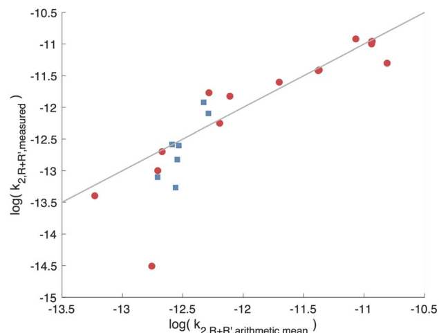
Fig. 5 The relationship between the cross-reaction rate coefficients and the arithmetic mean of the self-reaction rate coefficients ( k_2 ) for the peroxy radical systems given in Jenkin et al. 2019 (red circles), and the same relationship between k_2\alpha_{2d} values for the cross- and self-reactions examined in this study (blue squares). The solid gray line denotes the 1 : 1 line.
