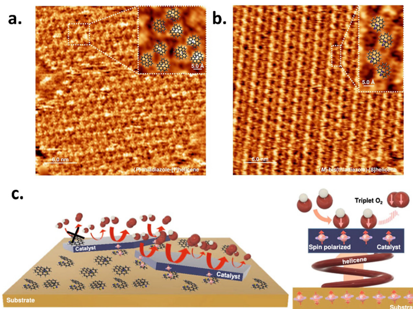
Fig. 3 Chirality-driven modulation of NiO x electrocatalysts: STM image of SAM of (a) (P)-thiadiazole-[7] helicene and (b) (M)-bis(thiadiazole)-[8] helicene. (c) Illustration of the effect of spin polarization employing the catalyst-chiral molecule-Au substrate configuration. The figure is adopted from ref. 18 with permission from Nature © 2022.
