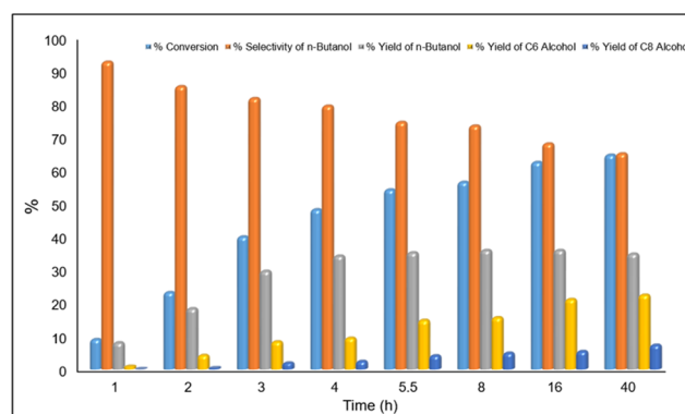
Fig. 9 Reaction profile for the 31 -catalysed ethanol upgradation reaction reported by Milstein and co-workers. 82
