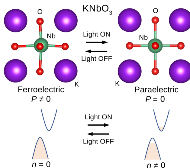
Fig. 1 Photoinduced phase transition in the perovskite oxide KNbO 3 . The ground state is a polar rhombohedral phase (space group R3m ). Upon photoexcitation, electrons are promoted to the conduction band ( n \neq 0 ) and KNO transforms into a nonpolar cubic phase (space group Pm\bar{3}m ), due to the screening of electrostatic dipole–dipole interactions. An analogous photoinduced phase transition occurs in the polar orthorhombic phase (space group Amm2 ) stabilized at T \geq 225 K.
