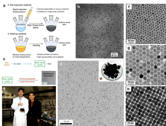
Fig. 7 (a) Schematic illustration of the hot-injection method and heat-up method for uniform-sized nanoparticles. (b) Transmission electron microscopy (TEM) image of 11 nm \gamma - \text{Fe}_2\text{O}_3 nanoparticles. (c) The overall scheme for the synthesis of monodispersed nanoparticles through metal-oleate complexation. (d) TEM image of 12 nm \text{Fe}_3\text{O}_4 nanoparticles. Inset is a photograph of 40 g of the monodispersed \text{Fe}_3\text{O}_4 nanoparticles, and a US one-cent coin for comparison. (e) Photograph of Taeghwan Hyeon and Jongnam Park in 2004. (f)–(h) TEM images of (f) 6 nm, (g) 12 nm, (h) 10 nm monodispersed \text{Fe}_3\text{O}_4 nanoparticles. Reproduced from ref. 44 with permission from Wiley, copyright 2023.
