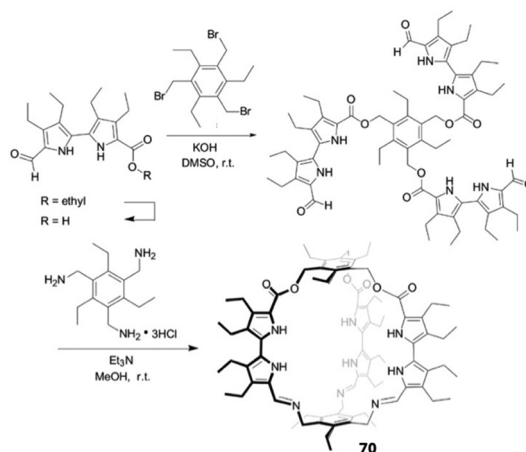
Fig. 36 Synthetic pathway toward hexapyrrrolic cage 70 , reported by Zhang et al.
