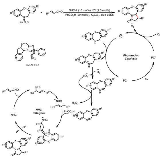
Scheme 16 Synthesis of pyrrolo[1,2- d ][1,4]oxazepin-3(2 H )-ones.
