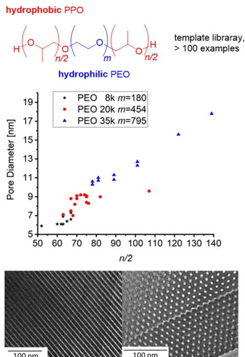
Fig. 3 Amphiphilic block copolyether series based on PEO macroinitiators with different molar masses for OMC/OMS preparation. Middle: correlation of n/2 and pore diameter (OMC). Bottom: TEM of OMC based on \text{PO}_{82}\text{-EO}_{454}\text{-PO}_{82} (9 nm pore diameter). Reproduced from ref. 104 with permission from American Chemical Society, copyright 2021.
