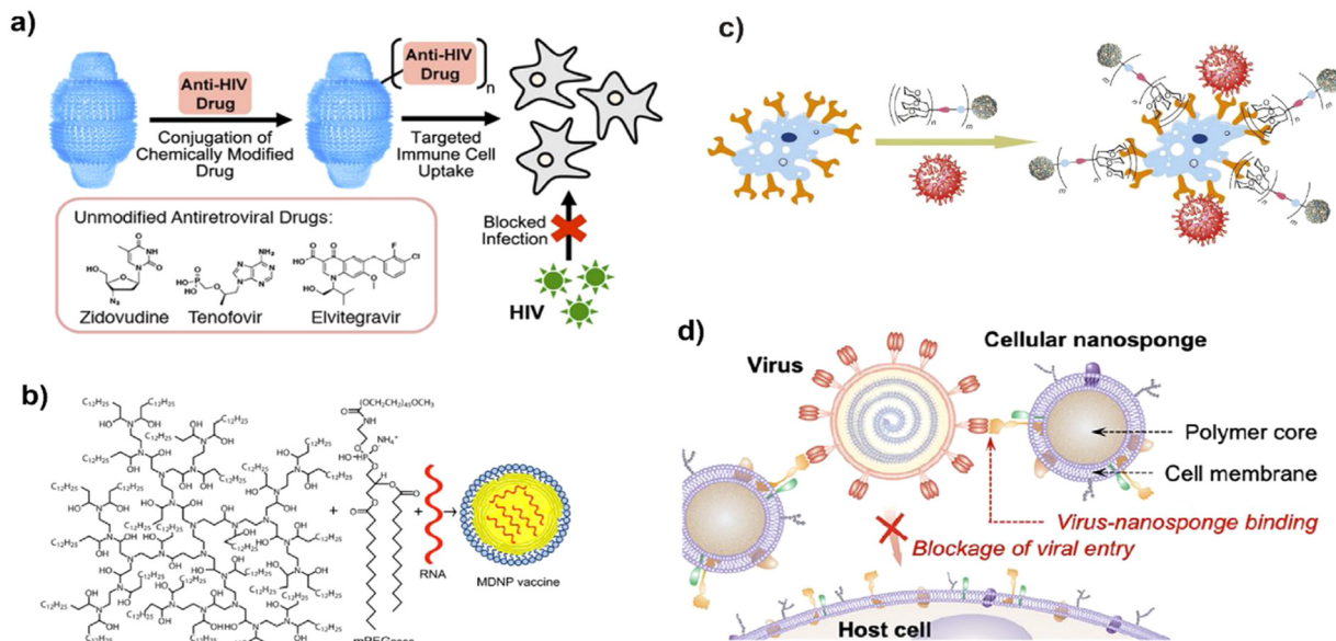
Fig. 3 Possible modes of the antiviral efficacy of nanotechnology. (a) Effect of antiviral drug delivery against HIV-1 infection, adapted from Fulcher et al. 36 Copyright 2019, American Chemical Society. (b) Schematic of vaccine delivery using lipid-derived dendrimer nanoparticles through m-RNA. Reproduced with permission from Chahal et al. 37 Copyright 2016, National Academy of Sciences, USA. (c) Blocking approach of virus-like glycodendrimer nanoparticles to the infection site, adapted from Ribeiro-Viana et al. 38 Copyright 2018, Nature Publishing Group. (d) Strategy of mimicking host cell membrane carrying nanodecoy host cell membrane for adsorbing Zika virus, adapted from Zhang et al. 39 Copyright 2020, American Chemical Society.
