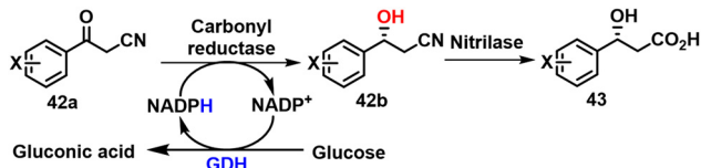
Scheme 21 The biosynthesis route to ( R )- \beta -hydroxy carboxylic acids.
