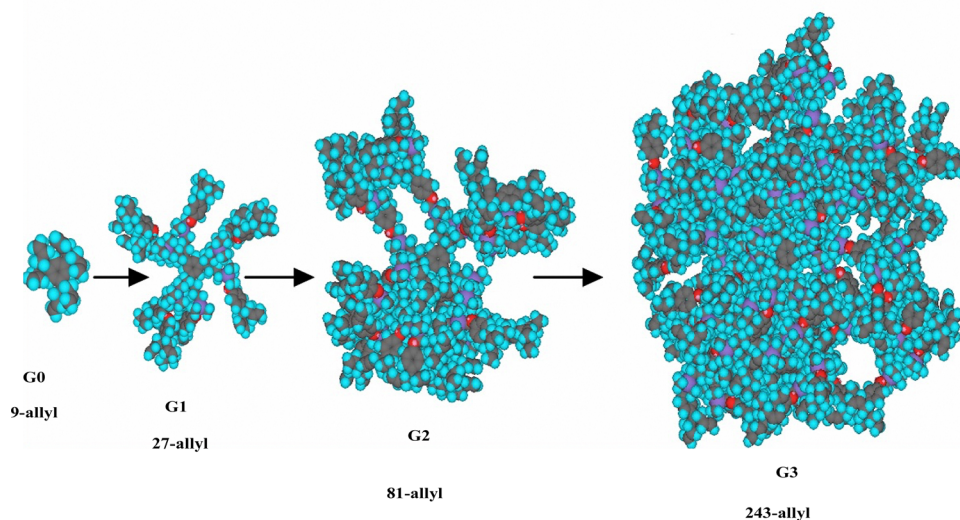
Fig. 3 Molecular modeling of the dendritic size progression from \text{G}_0 (9-allyl) to \text{G}_3 (243-allyl).
