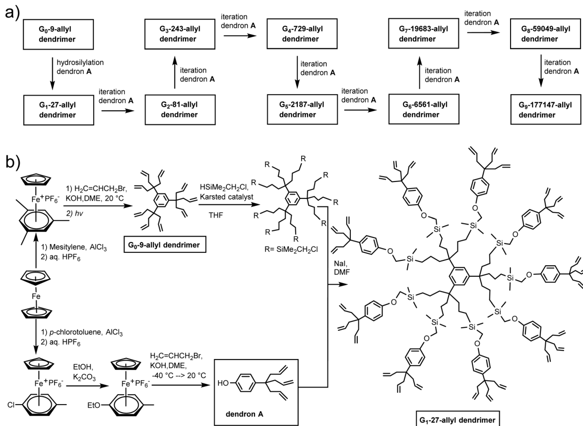
Scheme 6 \text{CpFe}^+ -induced arene activation for the synthesis of the \text{G}_0 -9-allyl dendritic core and dendron A towards the multiple-generation divergent construction of large poly-allyl-terminated dendrimers following 1 \rightarrow 3 branching until the 9th generation.
