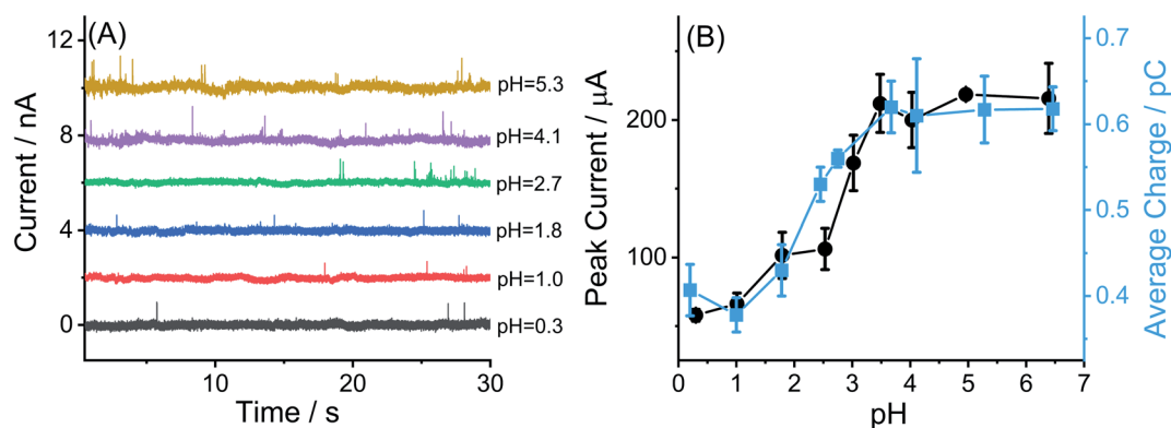
Fig. 7 (A) Representative chronoamperograms of a carbon micro-disc electrode immersed in a 1.0 M ( \text{pH} = 0.3 ) and 0.1 M \text{HNO}_3 ( \text{pH} = 1.0 ) and 0.1 M \text{KNO}_3 solutions at different pH values of 1.8, 2.7, 4.1 and 5.3 containing 0.01 \text{ g L}^{-1} MWCNTs- \text{NH}_2 at a potential of 1.90 V vs. SCE; (B) the comparison of oxidative peak current from CV (black dots) and average charge from oxidative spikes (blue dots) as a function of solution pH.
