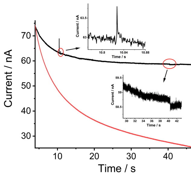
Fig. 6 Chronoamperograms of a carbon micro-disc electrode ( d = 33 \mu\text{m} ) immersed in a 0.1 M \text{KNO}_3 ( \text{pH} = 6.4 ) solution containing MWCNTs- \text{NH}_2 (black line) or not (red line) at a potential of 1.90 V vs. SCE. The inset is an enlarged view of impact spike and step at 1.90 V in the presence of MWCNTs- \text{NH}_2 .
