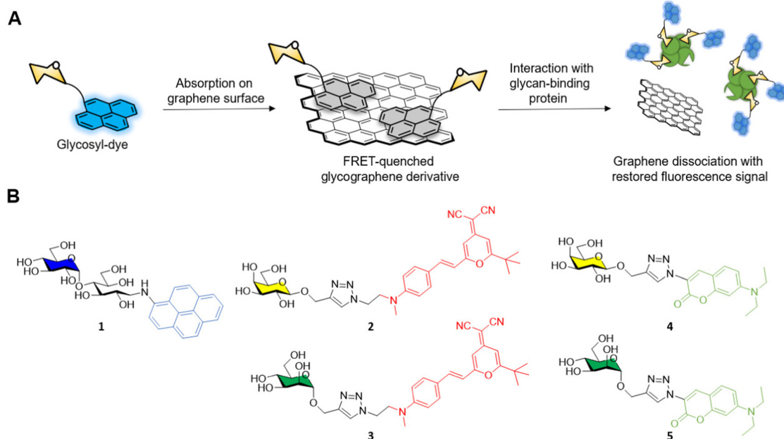
Fig. 1 (A) General principle for graphene and graphene derivatives-based FRET fluorescent glycoprobes used for glycan-binding protein sensing. (B) Structure of aminopyrene- 1 , dicyanomethylene- 2 and 3 , and aminocoumarin- 4 and 5 glycoside derivatives.
