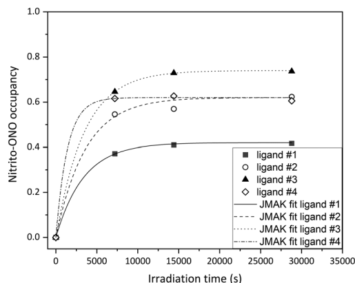
Fig. 6 ES nitrito-( \eta^1 -ONO) in polymorph I of 1 as a function of irradiation time with \lambda = 465 nm at 150 K; for ligand #1 \alpha_0 = 0 , \alpha_\infty = 0.42 , n = 1 and a value of k = (0.297 \pm 0.008) \times 10^{-3} \text{ s}^{-1} was refined from the data ( R^2 = 0.9998 ); for ligand #2 \alpha_0 = 0 , \alpha_\infty = 0.62 , n = 1 and a value of k = (0.277 \pm 0.037) \times 10^{-3} \text{ s}^{-1} was refined from the data ( R^2 = 0.9936 ); for ligand #3 \alpha_0 = 0 , \alpha_\infty = 0.74 , n = 1 and a value of k = (0.287 \pm 0.003) \times 10^{-3} \text{ s}^{-1} was refined from the data ( R^2 = 0.9999 ); for ligand #4 \alpha_0 = 0 , \alpha_\infty = 0.62 , n = 1 and a value of k = (0.707 \pm 0.342) \times 10^{-3} \text{ s}^{-1} was refined from the data ( R^2 = 0.9991 ).
