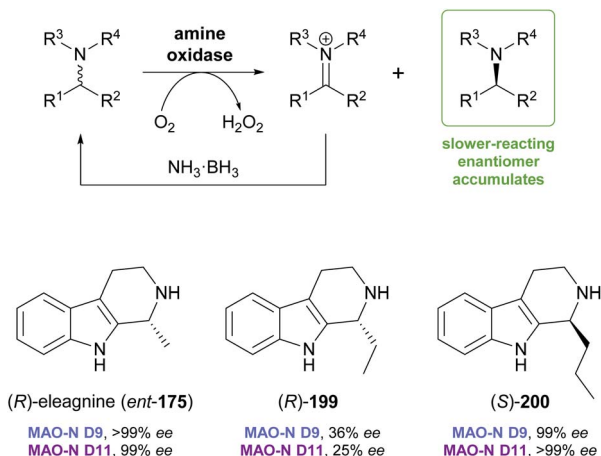
Scheme 24 General reaction scheme for the 'cyclic deracemisation' of amines, and examples of tetrahydro- \beta -carboline that have been deracemised using engineered variants of MAO-N.
