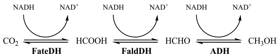
Fig. 1 The enzymatic conversion of CO 2 to methanol catalyzed by FateDH, FalDH and ADH.
