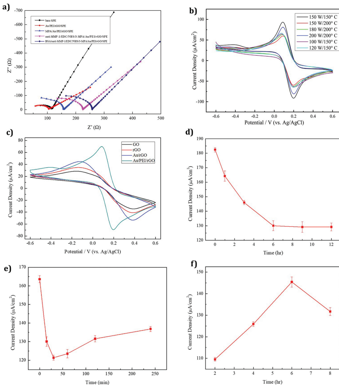
Fig. 5 (a) EIS spectra of different modified electrodes (conditions: 5 mM \text{Fe}(\text{CN})_6^{3-/4-} dissolved in 0.1 M PBS/0.1 M KCl (pH 7.4), scan rate 50 \text{ mV s}^{-1} ). (b) CVs of the AuNP/PEI/rGO-modified SPE (conditions: 5 mM \text{Fe}(\text{CN})_6^{3-/4-} dissolved in 0.1 M PBS/0.1 M KCl (pH 7.4), scan rate 50 \text{ mV s}^{-1} , n = 3 ) prepared under different microwave synthesis conditions. (c) CV responses of four different modified electrodes, namely GO, rGO, Au/rGO and AuNP/PEI/rGO-modified SPE. (d) Plot of the 3-MPA modification time versus current change. (e) Plot of the EDC/sulfo-NHS modification time (0, 15, 30, 60, 120, and 240 min) versus current change. (f) Plot of the MMP-1 antibody modification time versus current change.
