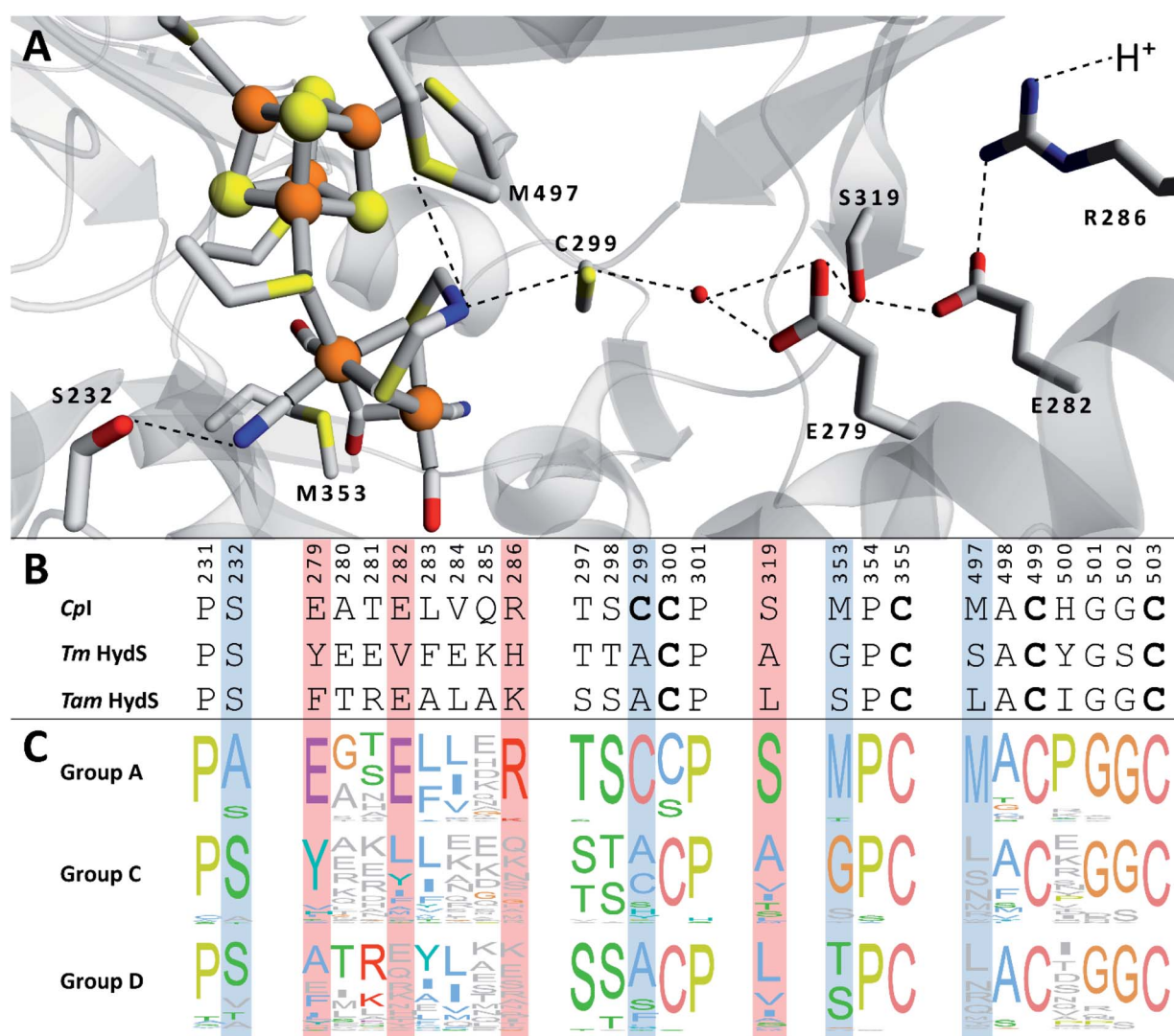
Fig. 1 (A) Structural view of the active site and proton transfer pathway of a prototypical [FeFe]-hydrogenase. Structure and numbering based on Cpl (PDB ID: 4XDC). Shown amino acid residues are either involved in interactions with the H-cluster or in the proton transfer pathway and show large variations between groups A, C and D. Potential interactions are shown with dashed lines. (B) Amino acid sequence comparison of Cpl , Tm HydS and Tam HydS ( Cpl numbering) based on a Clustal \Omega sequence alignment 60 of sequences retrieved from Greening et al. 2016 (ref. 7) and homology modeling. H-cluster interacting cysteine residues are highlighted in bold. (C) Normalized consensus logos of [FeFe]-hydrogenase groups A, C and D generated in Jalview using the sequence alignment in (B). Coloring is based on the Clustal X color scheme. Amino acid residues involved in H-cluster interaction and proton transfer that show variation between the groups are highlighted in blue and red, respectively.
