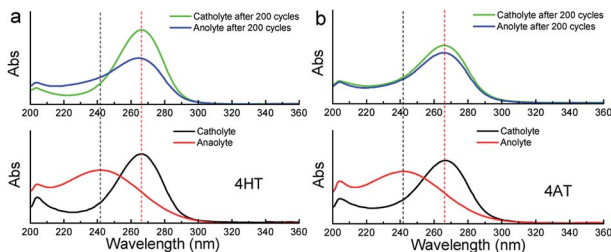
Fig. 7 Ultraviolet spectra of the anolyte and catholyte of the symmetric 4HT (a) and 4AT (b) RFBs, in 2 M KCl solution before and after 200 charge–discharge cycles.
