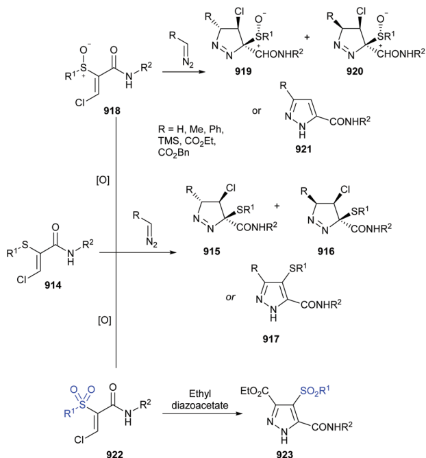
Scheme 132 [3 + 2]-dipolar cycloaddition of \alpha -sulfenyl/sulfinyl/sulfonyl- \beta -chloroacrylamides with electron rich and electron deficient diazoalkanes.
