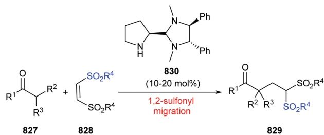
Scheme 121 Organocatalyst mediated 1,2-carbon to carbon sulfonfyl migration resulting from nucleophilic addition to bis activated vinyl-sulfones.
