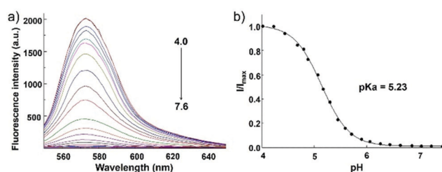
Fig. 3 (a) Fluorescence spectra of probe 2 ( 10 \mu\text{M} ) at various pH values in Britton–Robinson buffer solution ( 40 \mu\text{M} ), \lambda_{\text{ex}} = 525 \text{ nm} , (b) pH titration curve of probe 2 , \lambda_{\text{ex}} = 525 \text{ nm} , \lambda_{\text{em}} = 573 \text{ nm} . Copyright 2014 Elsevier.
