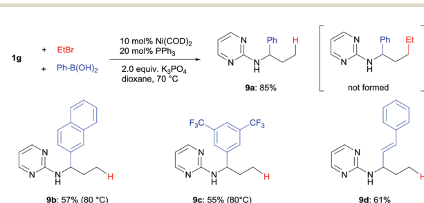
b) 1,3-Hydroarylation of internal alkenes
