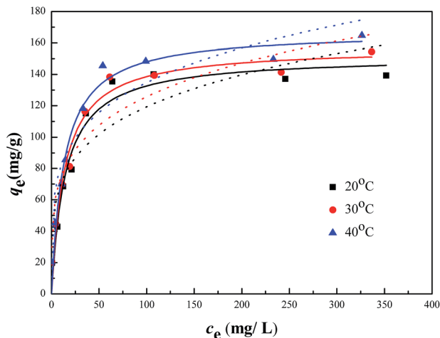
Fig. 9 Langmuir isotherm (solid line) and Freundlich isotherm (dash line) for the adsorption of Cr(vi) on CMB (reaction conditions: c_0 = 20\text{--}500 mg L -1 ; V = 50 mL; m = 50 mg; t = 6 h; \text{pH} = 2 ; T = 20, 30, 40 °C).
