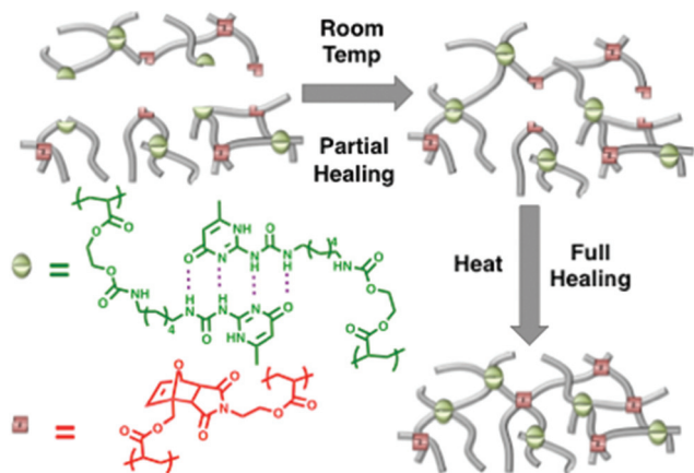
Scheme 1 Synthesis and proposed healing mechanism of the PHEA-FMIDA-UPyA material. Initially the hydrogen bonded UPy units join to partially heal the material. With thermal stimulus the covalently linked FMIDA units join across the interface.
