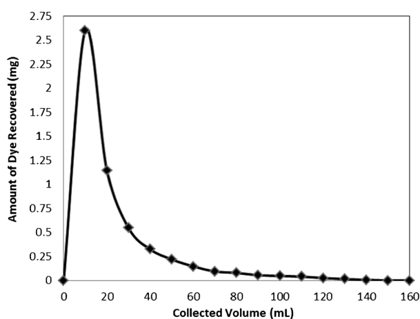
Fig. 11 Recovery of the dye Rose Bengal from the bottom ash column.
