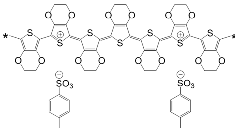
PEDOT:Tos
