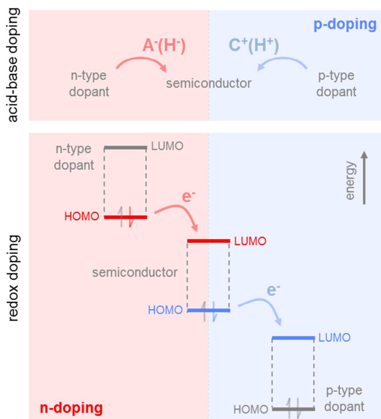
Fig 9. Basic principle of acid-base doping, which involves the transfer of an anion ( A^- , e.g. H^- ) or cation ( C^+ , e.g. H^+ ) to the semiconductor (top); and redox doping, which involves the transfer of an electron to the LUMO or from the HOMO of the semiconductor in case of n- and p-doping, respectively (bottom).
