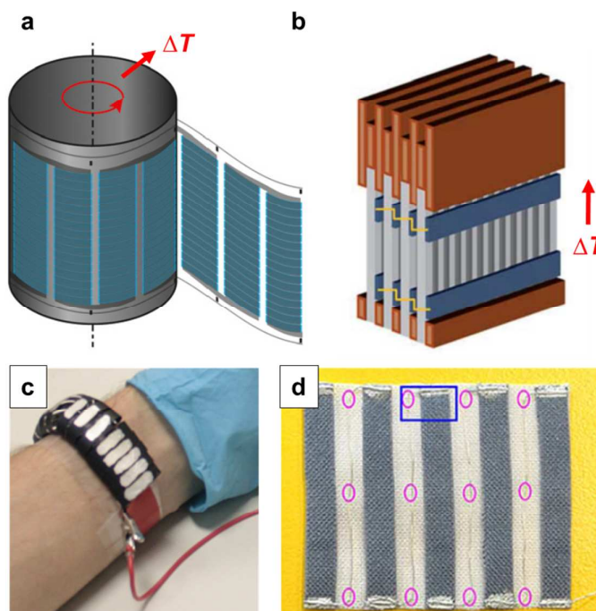
Fig 16. Possible designs of printed thermoelectric modules: (a) flexoprinted PEDOT:PSS based arrays on PET foil are rolled up into a cylinder; (b) screen-printed PEDOT:PSS based arrays on paper are sandwiched between copper plates and stacked into a module; (c) an array of n- and p-type legs is defined by selectively irradiating a carbon nanotube:P3HT composite with UV-light, followed by cutting and folded into a wearable toroidal device; (d) a textile-based thermoelectric generator of screen-printed PEDOT:PSS legs on a polyester fabric that are connected with conducting silver paste; images reproduced with permission from refs.1, 5, 6, 42, published by Wiley, the Royal Society of Chemistry, Wiley and the Nature Publishing Group, respectively.
