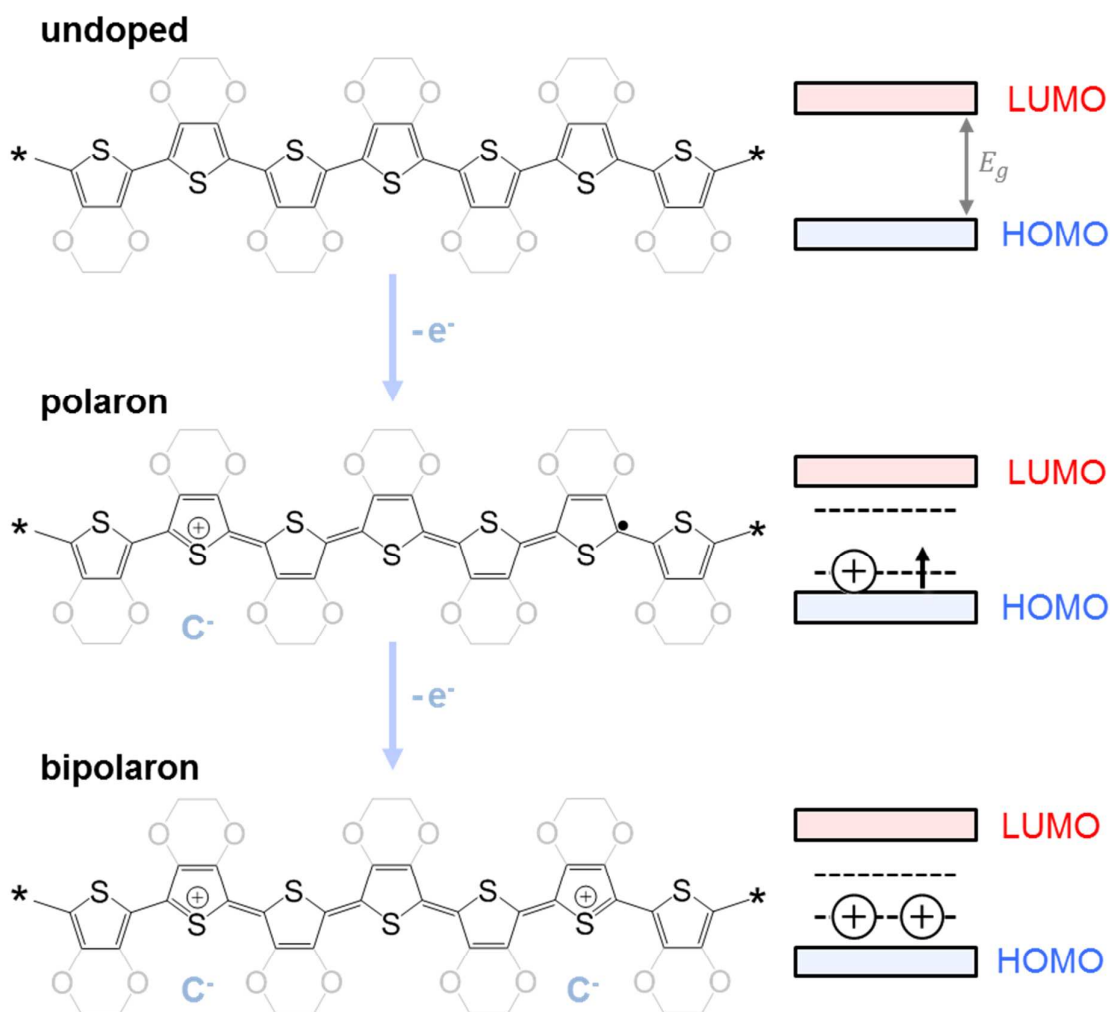
Fig. 4. Schematic for p-doping of polythiophene and PEDOT (left) and corresponding band structure evolution (right): electron transfer ( -e^- ) to the undoped polymer (top) leads to the formation of a polaron (middle) and finally a bipolaron state (bottom); counterions ( C^- ) ensure charge neutrality.
