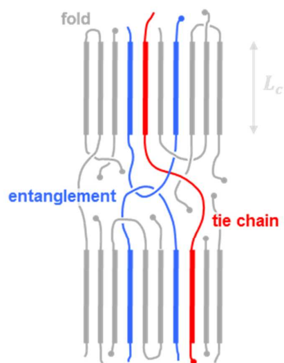
Fig 7. Schematic nanostructure of a semi-crystalline polymer, indicating a chain fold that re-enters the same crystallite, a tie chain that bridges two adjacent crystallites, and a chain entanglement that is trapped in the amorphous region between two crystallites.
