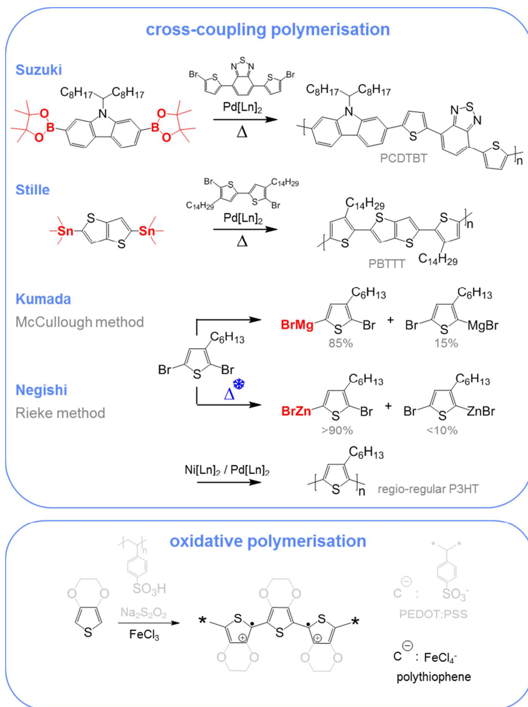
Fig. 5. Most common reaction schemes for conjugated polymer synthesis include cross-coupling polymerisations (top), where a bifunctionalised monomer (red, boronic ester for Suzuki, organostannyl for Stille, Grignard for Kumada and organozinc for Negishi) is polymerised with an aryl halide (mostly an aryl bromide) by action of a metal catalyst, and oxidative polymerisation (bottom) of polythiophene (black) and polydioxo thiophene (grey).
