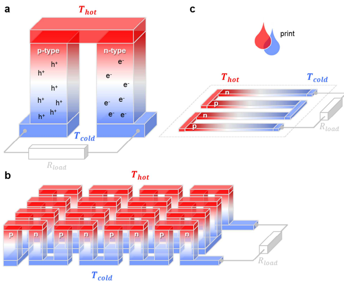
Fig. 1. Schematics of (a) a thermoelectric element, which comprises an n- and p-type thermoelectric leg that experience a temperature gradient \Delta T = T_{hot} - T_{cold} leading to charge accumulation at the cold ends, (b) a conventional thermoelectric module that comprises an array of elements, which are connected electrically in series but thermally in parallel, and (c) an in-plane (printable) array of elements. A load resistance R_{load} is connected to close the circuit, resulting in maximum power generation when R_{load} = R_{in} but maximum power conversion efficiency when R_{load} = R_{in}\sqrt{1 + ZT} (cf. equations 7 and 8).
