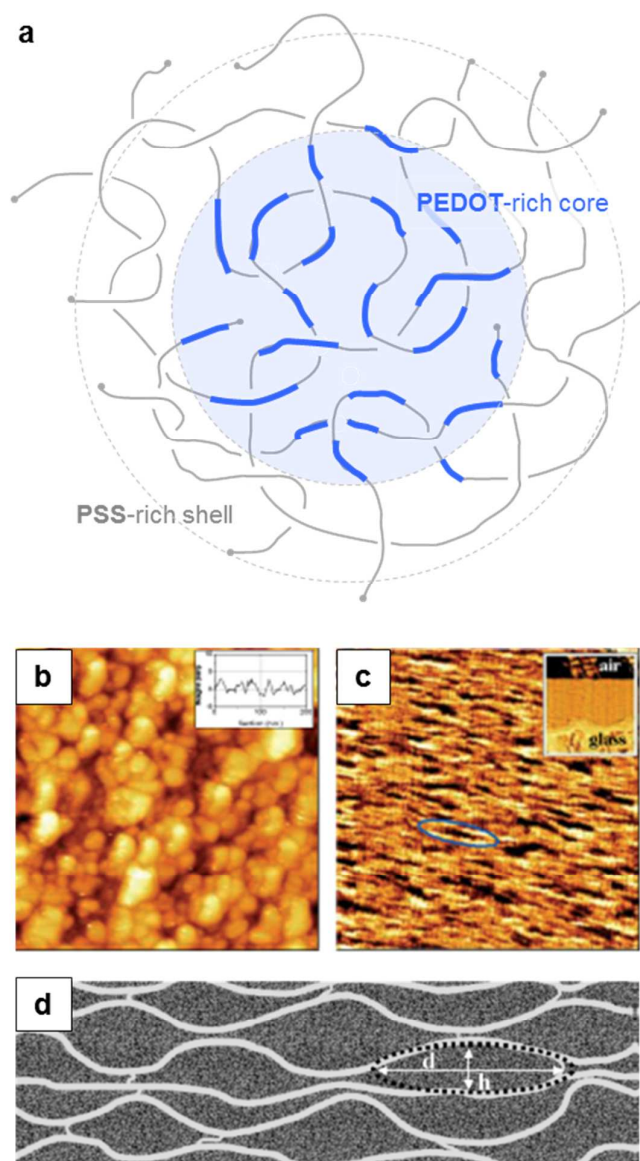
Fig 14. Nanostructure of PEDOT:PSS. (a) Core-shell structure of a PEDOT:PSS complex in an aqueous dispersion; (b) scanning tunnelling microscopy image of a PEDOT:PSS film surface; (c) cross-sectional atomic force microscopy image of a cleaved PEDOT:PSS film; (d) schematic of PEDOT-rich clusters separated by PSS lamellae ( d = 20 to 25 nm, h = 5 to 6 nm); images reproduced with permission from ref. 48, published by Wiley.
