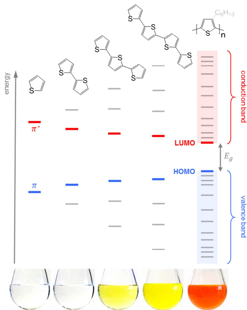
Fig. 3. Evolution of the HOMO and LUMO levels as well as bandgap E_g with increasing number of thiophene repeat units, resulting in a valence and conduction band for polythiophene; images of 5 g L -1 solutions in chloroform illustrate the narrowing of E_g , which leads to a red-shift in absorption (the polymer is P3HT). Note that crystallisation will lead to a further decrease in E_g due to delocalisation across adjacent chain segments.
