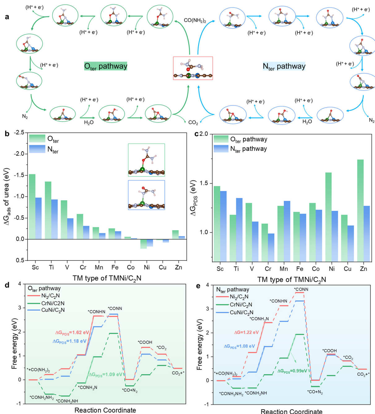
Fig. 2 (a) The schematic diagram of the O ter pathway and N ter pathway. (b) The urea adsorption free energy (ΔG ads ) on TMNi/C 2 N and the insets are the adsorption model of urea with O ter (green) and N ter (blue) structures, respectively. (c) The free energy change of potential determining steps (ΔG PDS ) of the two pathways on TMNi/C 2 N. (d and e) The free energy diagrams of the O ter and N ter pathway on Ni 2 /C 2 N, CrNi/C 2 N and CuNi/C 2 N, respectively.
