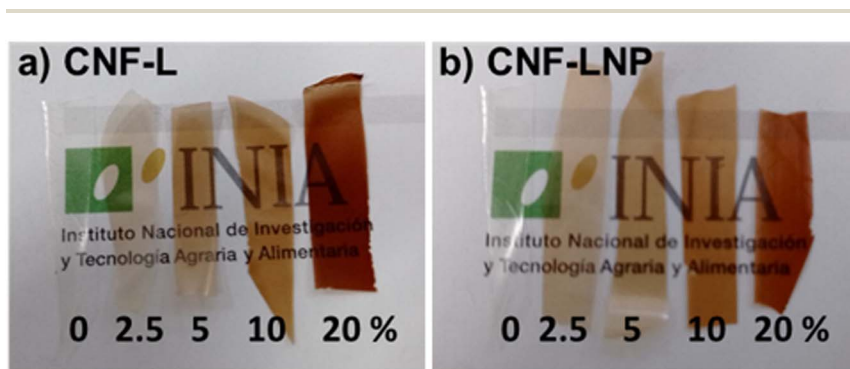
Fig. 1 Nanocellulose–lignin films with bulk lignin (a) and lignin nanoparticles (b). The lignin content of each film is indicated in the bottom of the images.
