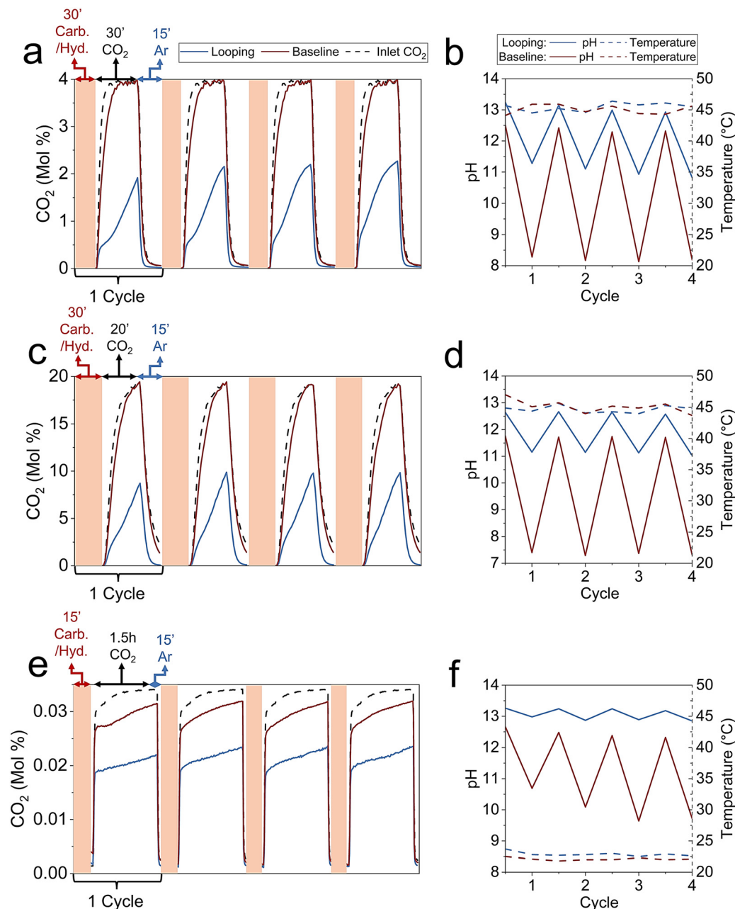
Fig. 2 (a) Four \text{Na}_2\text{CO}_3 looping cycles of 4% \text{CO}_2 with quenched BOF slag compared to the baseline; the conditions were 1 g slag per cycle, 45 ^{\circ}\text{C} , and 90 sccm 4% \text{CO}_2/\text{Ar} . (b) pH and temperature after each step in 4% \text{CO}_2 looping and baseline. Half cycles are after carbonation and full cycles are after \text{CO}_2 capture. (c) Four \text{Na}_2\text{CO}_3 looping cycles of 20% \text{CO}_2 with aged fines BOF slag compared to the baseline; the conditions were 10 g slag per cycle, 45 ^{\circ}\text{C} , and 90 sccm 20% \text{CO}_2/\text{Ar} . (d) pH and temperature after each step in 20% \text{CO}_2 looping and baseline. (e) Four \text{Na}_2\text{CO}_3 looping cycles of air \text{CO}_2 with quenched BOF slag compared to the baseline; the conditions were 0.05 g slag per cycle, 24 ^{\circ}\text{C} , and 90 sccm 343 ppm \text{CO}_2 . (f) pH and temperature after each step in air \text{CO}_2 looping and baseline.
