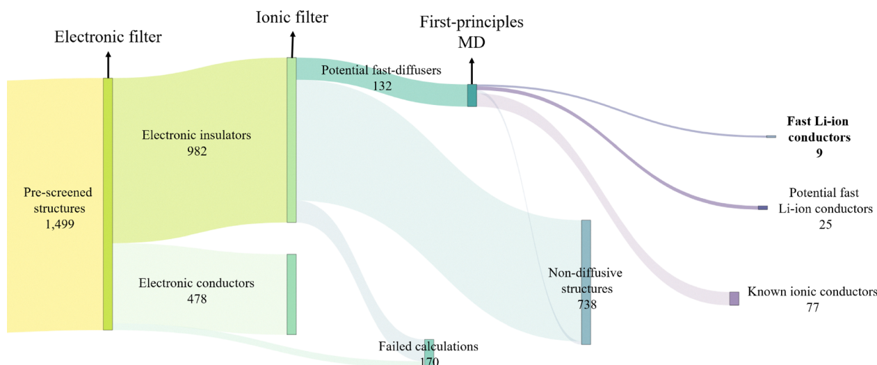
Fig. 5 Flowchart of the remaining workflow that only shows electronic structure calculations. Beginning with 1499 pre-screened structures, 9 most promising candidates are identified. Each node represents a filter based on ab initio methods that eliminates undesirable structures (indicated by lighter shaded links), while potentially suitable structures advance to the next filter (indicated by darker shaded links). The link thickness corresponds to the number of structures passing through each filter.
