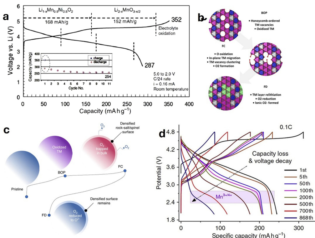
Fig. 6 (a) Voltage curve in the 1st cycle. Reproduced with permission from ref. 52. Copyright 2021, Chinese Society of Particuology and Institute of Process Engineering, (b) atomic-scale changes to ordering within the TM layer. BOP means the beginning of plateau, FC means full charge, FD means full discharge, and (c) macroscale changes to the cathode particles. Reproduced with permission from ref. 163. Copyright 2020, The Authors. (d) Cycling performances. Reproduced with permission from ref. 52. Copyright 2021, Chinese Society of Particuology and Institute of Process Engineering.
