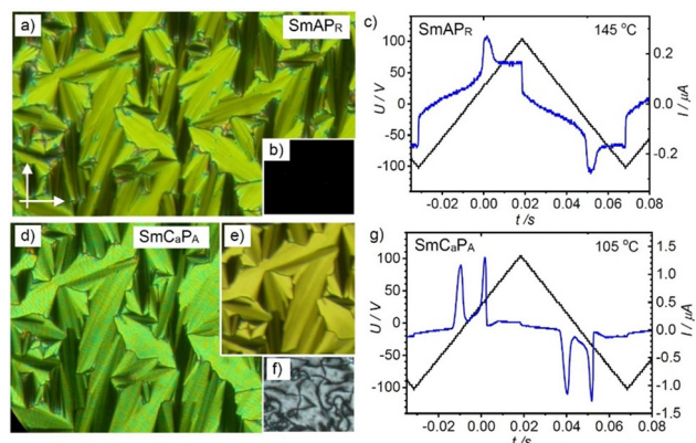
Fig. 5 POM textures (left) and polarization current response curves (right) of compound 1/O8 : (a)–(c) in the \text{SmAP}_R phase at 145 °C and (d)–(f) in the \text{SmCaPA} phase at 105 °C, (a) and (d) showing planar textures (PI coated ITO cell 6\ \mu\text{m} ) in (a) and (d) without applied field and in (e) under an applied field of +10\ \text{V}\ \mu\text{m}^{-1} ; (b) and (f) show the homeotropic textures without applied field, for additional data, see Fig. S28 (ESI † ).
