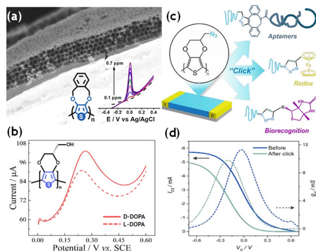
Fig. 6 (a) SEM image of the cross-section of a highly ordered macroporous PPDOT electrode. Inset shows a square wave anodic stripping voltammetry obtained during the successive addition of \text{Cu}^{2+} in a 10% diluted mezcalt solution. Adapted from ref. 221 with permission from the American Chemical Society, copyright 2018. (b) Differential pulse voltammetry curves of (S)-PEDTM modified electrodes in a solution containing D- or L-DOPA. Adapted from ref. 223 with permission from The American Chemical Society, copyright 2017. (c) Chemical structure of the poly-azidomethyl-EDOT (PEDOT- \text{N}_3 ) deposited between the drain and source electrodes to generate OECTs, and the schematic representation of the possible click functionalization with redox probes and biorecognition elements. (d) Threshold voltage and maximum transconductance for a PEDOT- \text{N}_3 OECT before and after the click reaction with ethynyl-ferrocene. Adapted from ref. 239 with permission from The American Chemical Society, copyright 2022.
