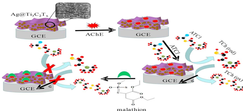
Fig. 7 Synthesis route of Ag@Ti 3 C 2 T x for the detection of the organophosphate pesticide malathion. Reproduced from ref. 106. Copyright (2018), adopted with permission from Elsevier.
